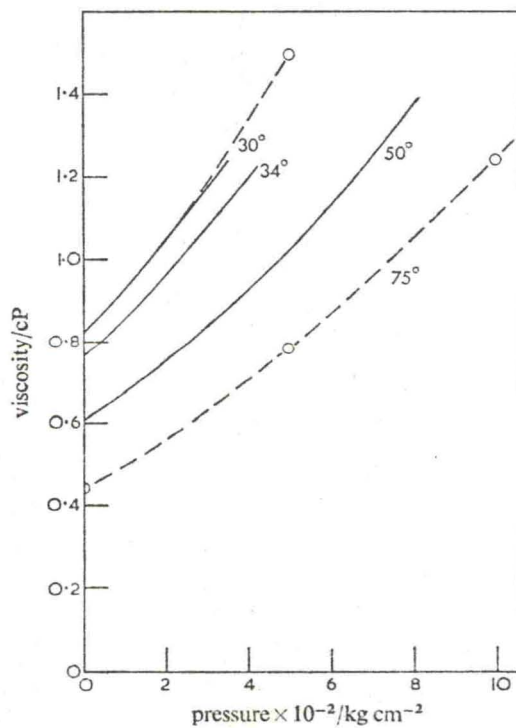
FIG. 7.—The viscosity of cyclohexane. ○, Bridgman 7 ; —, this work.
